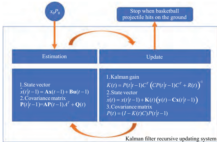
Fig. 2. The Kalman filter recursive updating system
