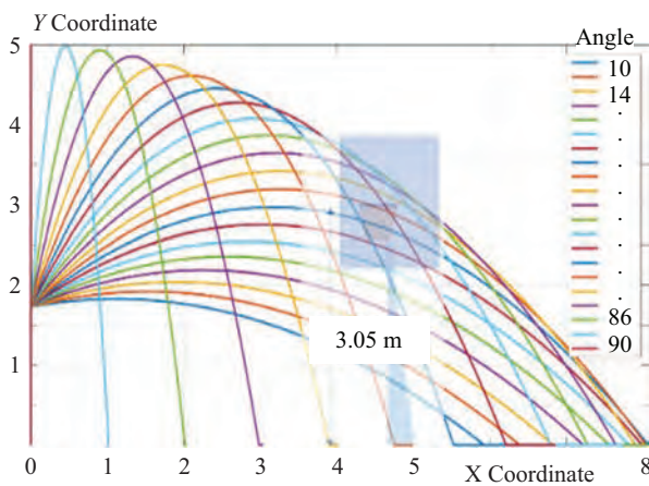
Fig. 12. Possible projectile trajectory
