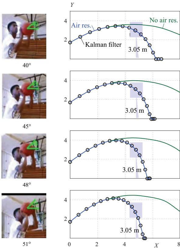
Fig. 13. Best possible projectile trajectories
