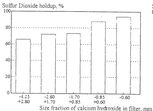
Figure 3 Effect of particle size fractions of \text{Ca}(\text{OH})_2 pellets in the filter on holdup.
