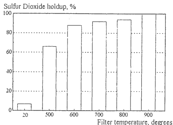
Figure 4. Effects of burning temperature on \text{SO}_2 holdup.
