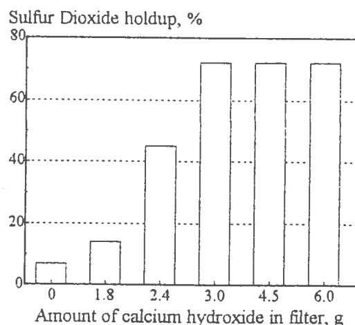
Figure 2. Effect of weight ratio of \text{Ca}(\text{OH})_2 filter to coal on \text{SO}_2 holdup.
