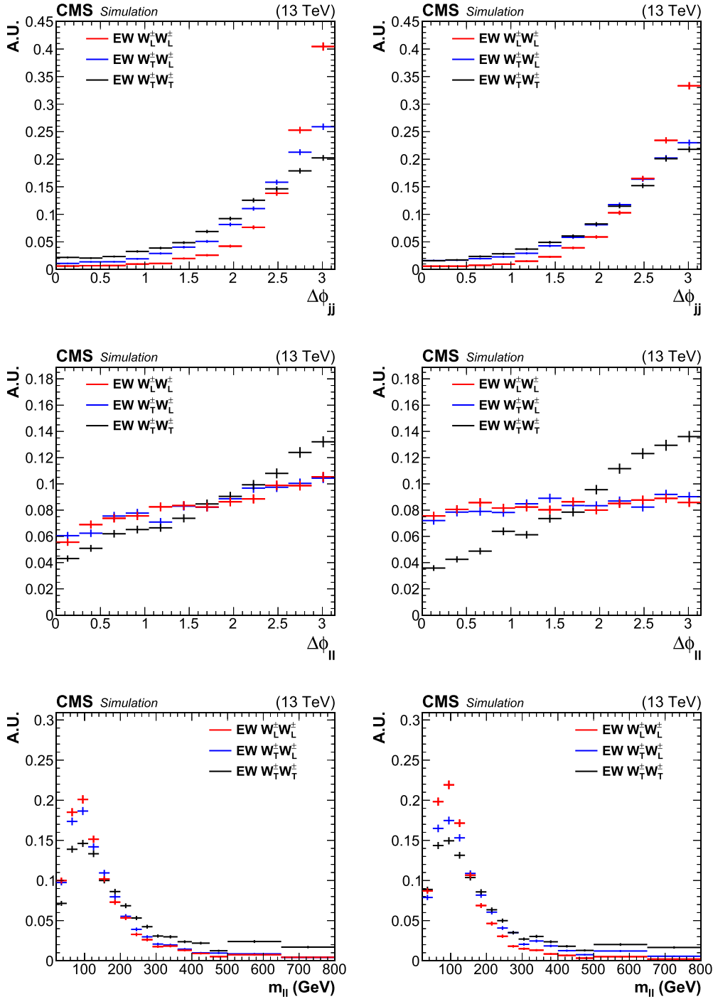
Fig. 2. Generator level distributions of \Delta\phi_{jj} (upper), \Delta\phi_{\ell\ell} (center), and m_{\ell\ell} (lower) in the fiducial region for the W_L^\pm W_L^\pm , W_L^\pm W_T^\pm , and W_T^\pm W_T^\pm processes with the helicity eigenstates defined in the parton-parton (left) and W^\pm W^\pm (right) center-of-mass reference frames. The distributions are normalized to unit area. The error bars represent the uncertainties associated with the limited numbers of simulated events.
