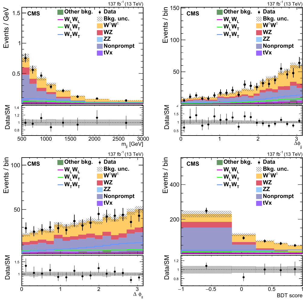
Fig. 3. Distributions of the m_{lij} (upper left), \Delta\phi_{lij} (upper right), \Delta\phi_{\ell\ell} (lower left), and of the output score of the inclusive BDT (lower right) in the W^\pm W^\pm SR. The predicted yields are shown with their best fit normalizations from the simultaneous fit. The histograms for the W^\pm W^\pm process include the contributions from the W_L^\pm W_L^\pm , W_L^\pm W_T^\pm , and W_T^\pm W_T^\pm processes (shown separately as solid lines), QCD W^\pm W^\pm , and interference. The histograms for other backgrounds include the contributions from double parton scattering, VVV, and from oppositely charged dilepton final states from t\bar{t} , tW , W^+ W^- , and Drell-Yan processes. The overflow is included in the last bin. The bottom panel in each figure shows the ratio of the number of events observed in data to that of the total SM prediction. The gray bands represent the uncertainties in the predicted yields. The vertical bars represent the statistical uncertainties in the data.
