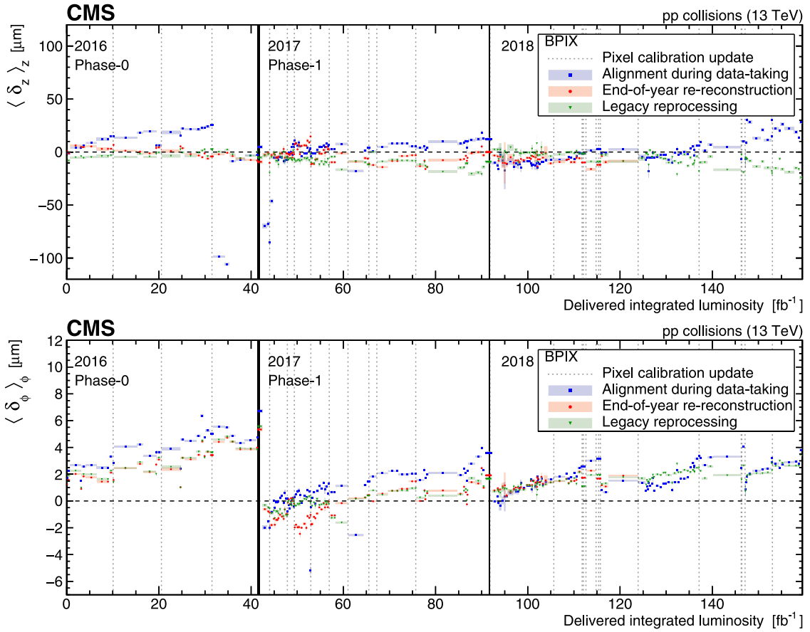
Fig. 33. The upper (lower) figure shows the mean difference in residuals in the z ( \phi ) direction for modules overlapping in the z ( \phi ) direction in the BPIX, \langle \delta_z \rangle ( \langle \delta_\phi \rangle ), as a function of the delivered integrated luminosity. The error bars show the statistical uncertainty in the mean of distribution of the residuals. These residuals are calculated using a sample of data recorded with the inclusive L1 trigger.
