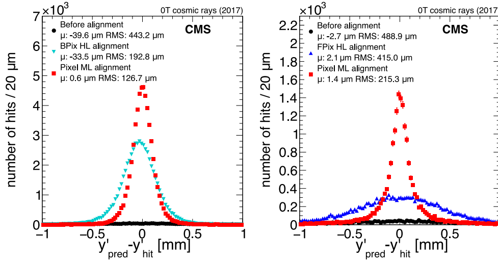
Fig. 16. Unbiased track-hit residuals in the BPIX (left) and FPIX (right), in the local y ( y' ) coordinate. The distributions are shown for the different alignment iterations that were performed: the black circles indicate the geometry assumed before performing any alignment fit, the blue and cyan triangles show the high-level (HL) structures alignment of the barrel and forward pixel detectors, and the red squares represent the module-level (ML) alignment of the pixel detector. The mean ( \mu ) and RMS of the distributions are given in the legend. Vertical error bars represent the statistical uncertainty; they are smaller than the marker size in most of the cases.
