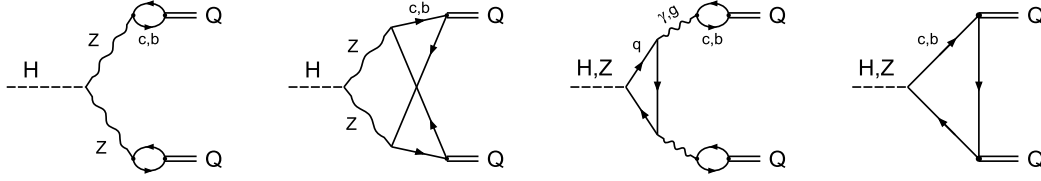
Fig. 1. Feynman diagrams for H \rightarrow QQ and Z \rightarrow QQ with Q = \text{charmonium or bottomonium states} . In the two leftmost diagrams [14], the virtual particles are Z bosons. The center-right diagram depicts indirect processes in the case where the flavor of the quark q in the loop is top, and direct processes in the case where it is charm or bottom. The other virtual particles are either photons or gluons. In the latter case additional soft-gluon exchange occurs. The rightmost diagram shows direct processes for the Higgs or Z bosons.
